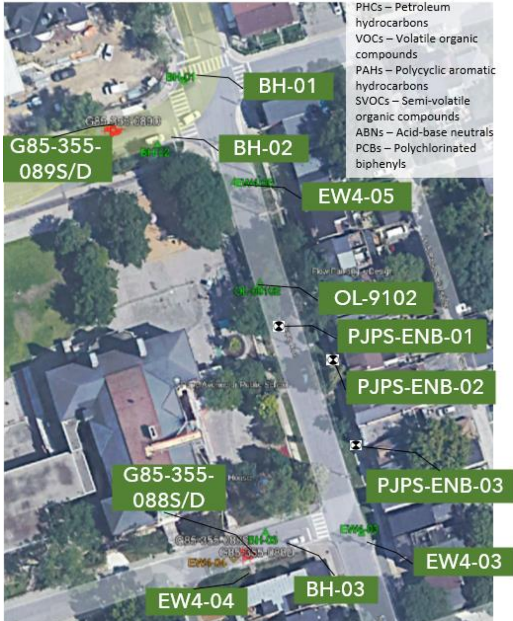
Figure 9-1 Geotechnical Borehole Locations
