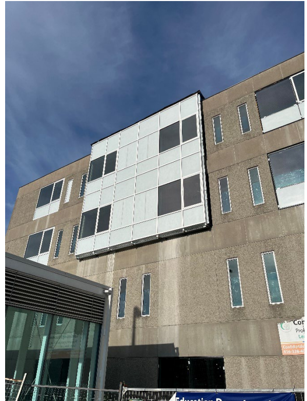
Zone B – Photo looking south and west at new façade and window installation.
