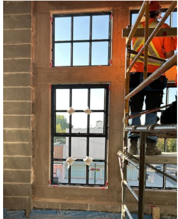
Zone A – Photo of south façade exterior and interior steel sash window installation
