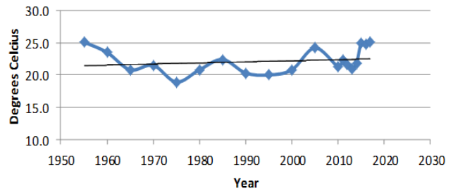
Sept: Average Daily Max Temperature
