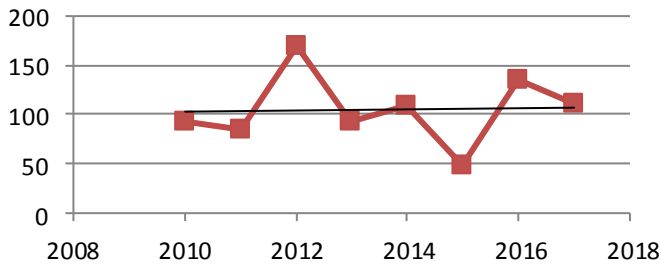
June: Number Of Cooling Degree Days
