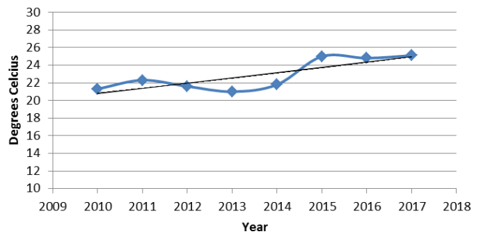
Sept: Average Daily Max Temperature
