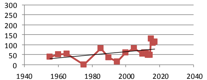
September: Number Of Cooling Degree Days
