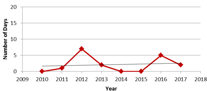
June: Number of Days with Daily Max Temp Over 31°C
