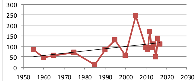
June: Number Of Cooling Degree Days
