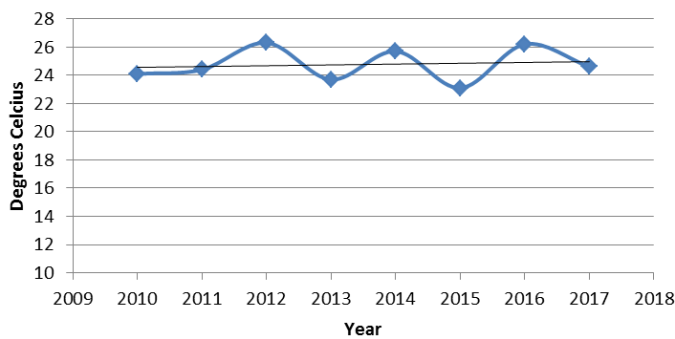
June: Average Daily Max Temperature
