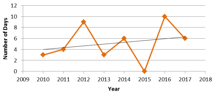
June: Number of Days with Daily Max Temp Over 28°C
