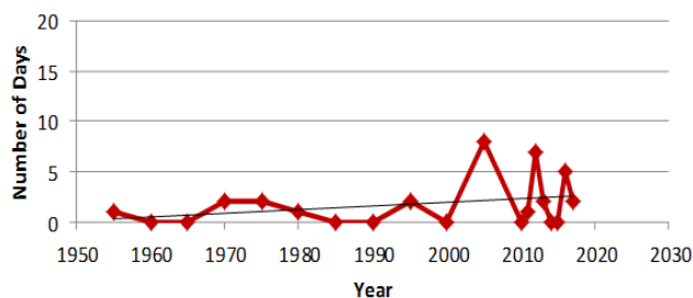
June: Number of Days with Daily Max Temp Over 31°C
