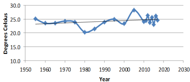
June: Average Daily Max Temperature
