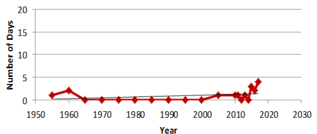
Sept: Number of Days with Daily Max Temp Over 31°C
