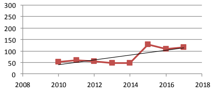
September: Number Of Cooling Degree Days
