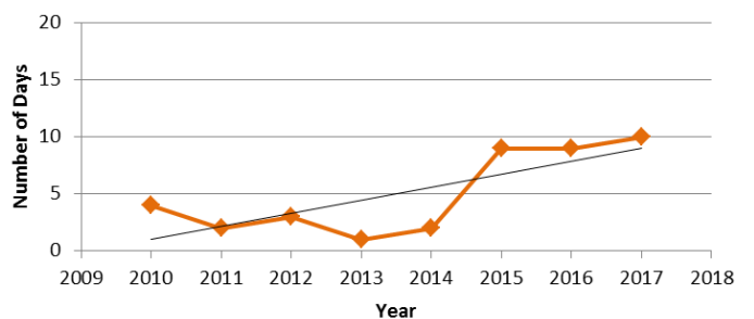
Sept: Number of Days with Daily Max Temp Over 28°C
